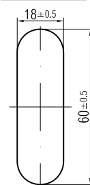
Detail Loch M
